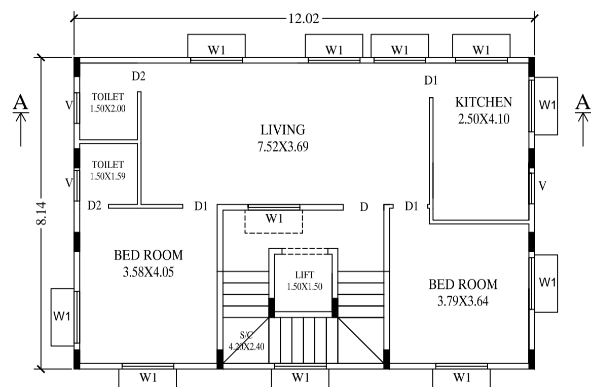
PROPOSED TYPICAL FIRST AND SECOND FLOOR PLAN
